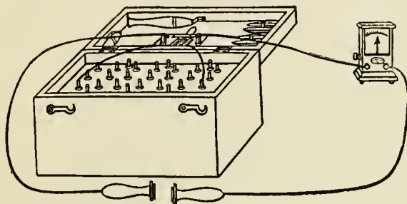
DIAGRAM SHOWING THE METHOD OF USING THE MILLIAMPÈRE-METRE.
